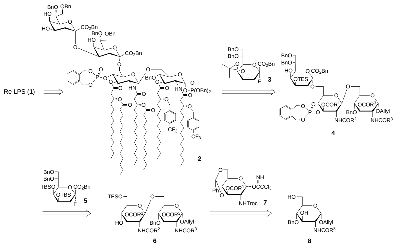
Scheme 1. Retrosynthesis of Re LPS (1). The tetrasaccharide backbone was constructed by sequential glycosylation reactions starting from terminal glucosamine 8. Bn = benzyl, R 1 COOH = ( R )-3-(tetradecanoyloxy)tetradecanoic acid, R 2 COOH = ( R )-3-(dodecanoyloxy)tetradecanoic acid, R 3 COOH = ( R )-3-(4-(trifluoromethyl)benzyloxy)tetradecanoic acid.
