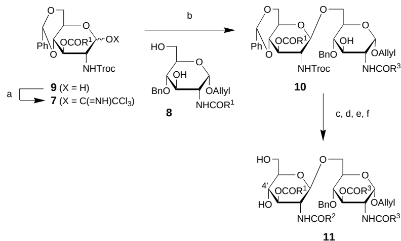
Scheme 2. Synthesis of lipid A moiety 11. a) Dowex 1-X8 (OH - form) in MicroKan, CCl 3 CN, CH 2 Cl 2 , 3 h (100%); b) Nafion-TMS, MS4A, CH 2 Cl 2 /perfluorohexane (3/1), 24 h (73%); c) ( R )-3-(4-(trifluoromethyl)benzyloxy)tetradecanoic acid, DCC, DMAP, CH 2 Cl 2 , 22 h (85%); d) Zn–Cu, AcOH, 1.5 h; e) ( R )-3-(dodecanoyloxy)tetradecanoic acid, DCC, CH 2 Cl 2 , 18 h (85% over two steps); f) TFA, H 2 O, CH 2 Cl 2 , 2 h (90%). DCC = dicyclohexylcarbodiimide, DMAP = 4-(dimethylamino)pyridine, MS4A = molecular sieves (4 Å), TFA = trifluoroacetic acid.
